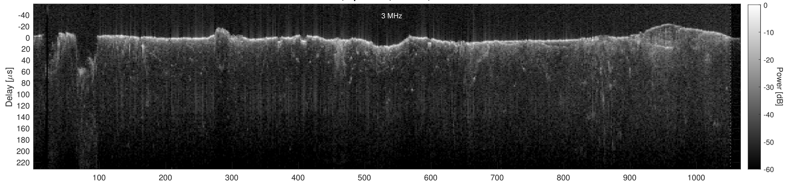
Orbit 2803, Cluttergram
