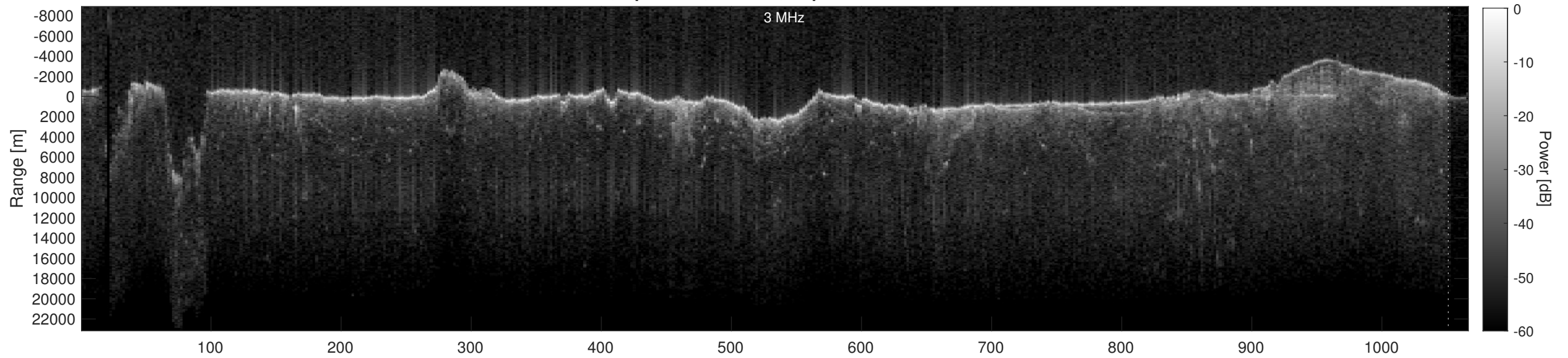
Orbit 2803, Depth-Corrected Cluttergram
