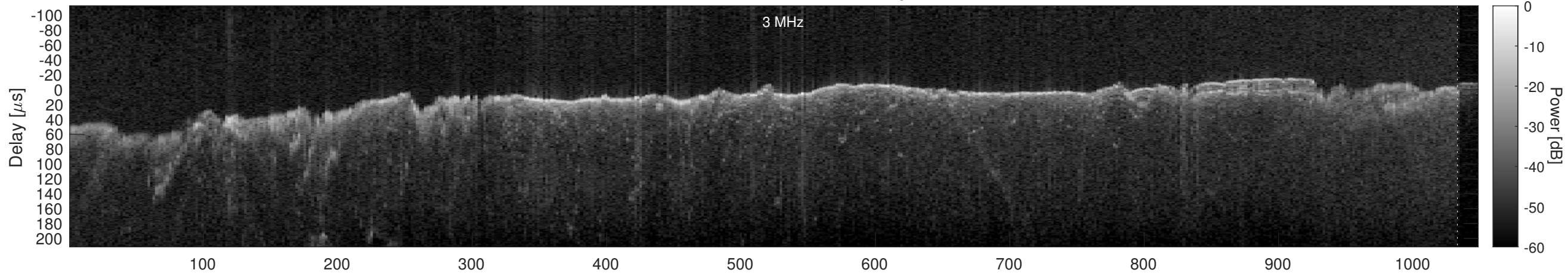
Orbit 2804, Window, Channel 2, Optimized
