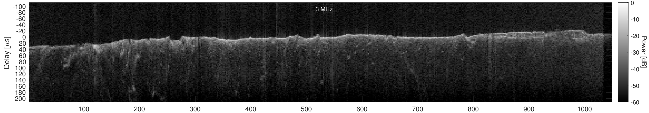
Orbit 2804, Cluttergram
