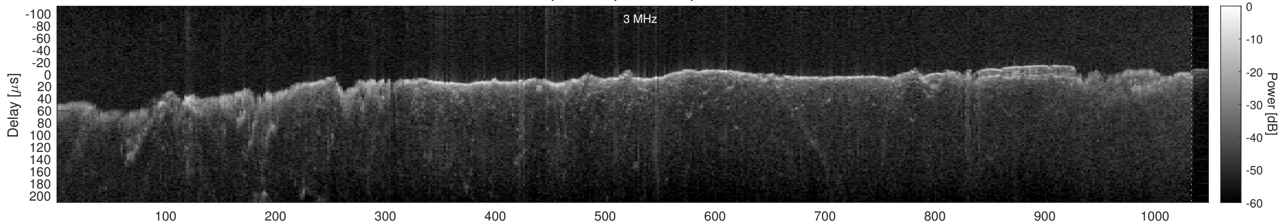
Orbit 2804, Window, Channel 2, Chapman
