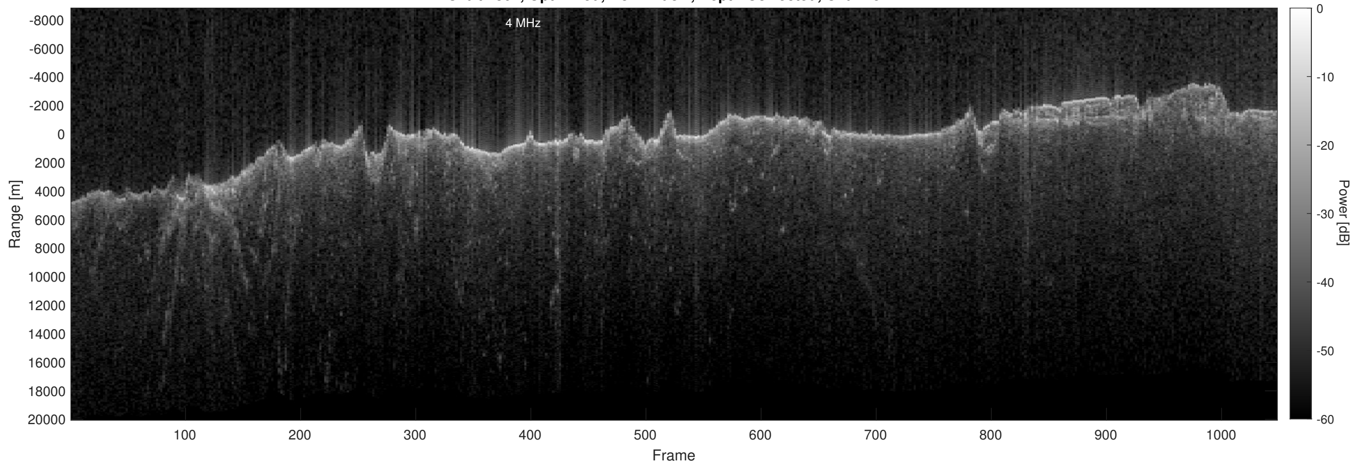
Orbit 2804, Optimized, No Window, Depth-Corrected, Channel 2
