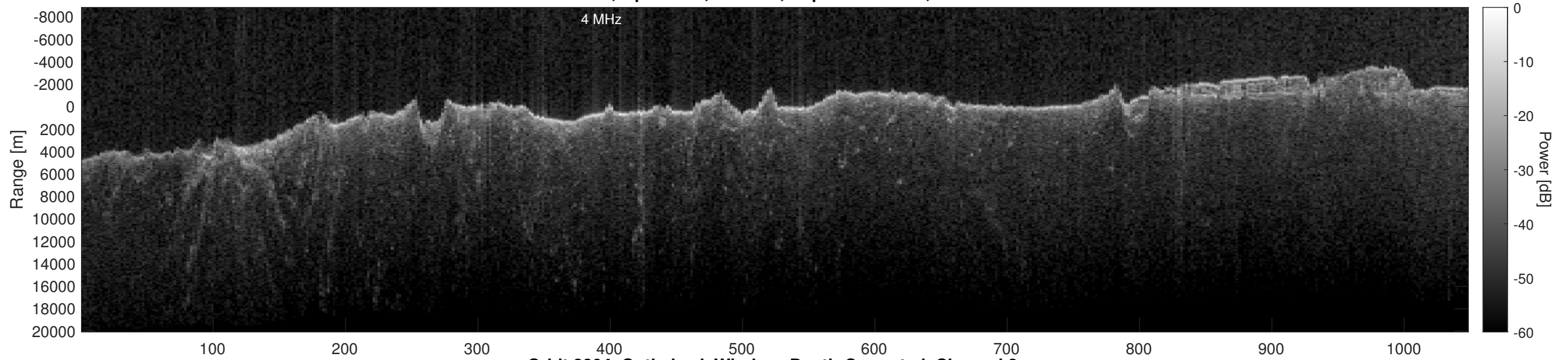
Orbit 2804, Optimized, Window, Depth-Corrected, Channel 2
