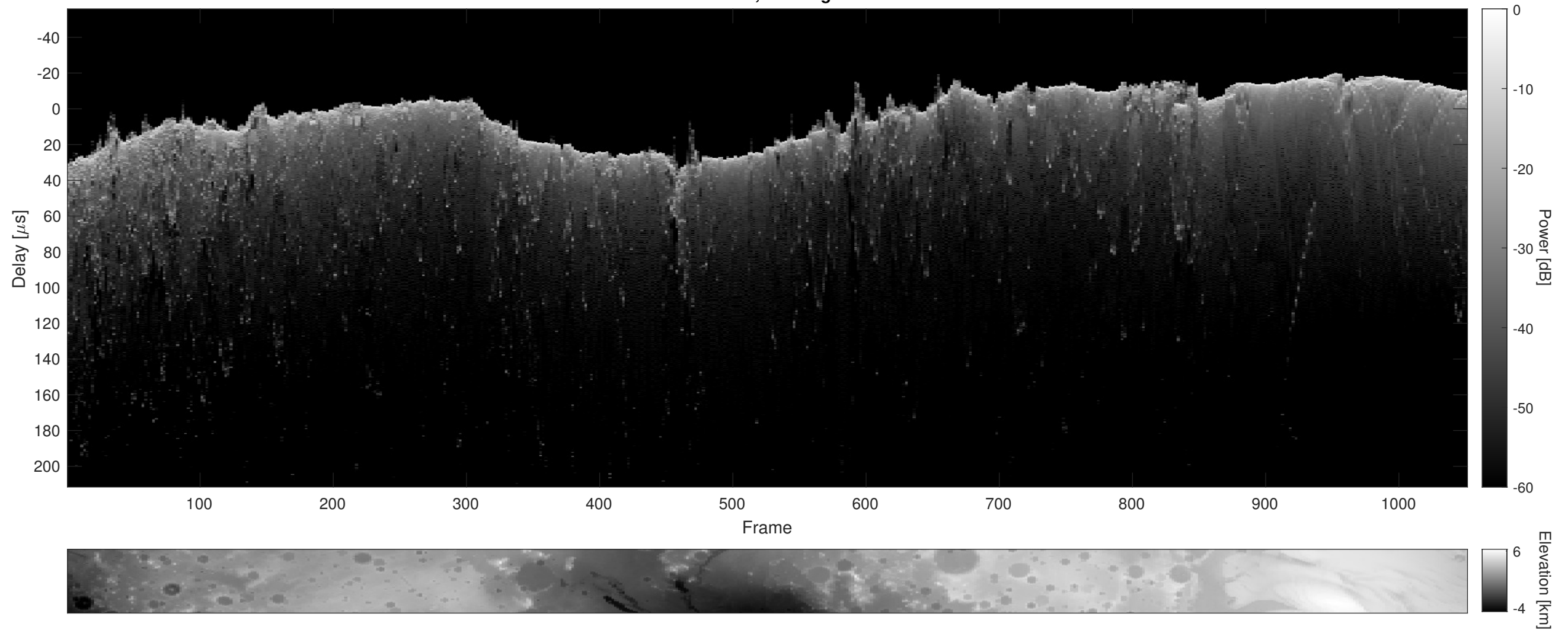
Orbit 2805, Cluttergram
