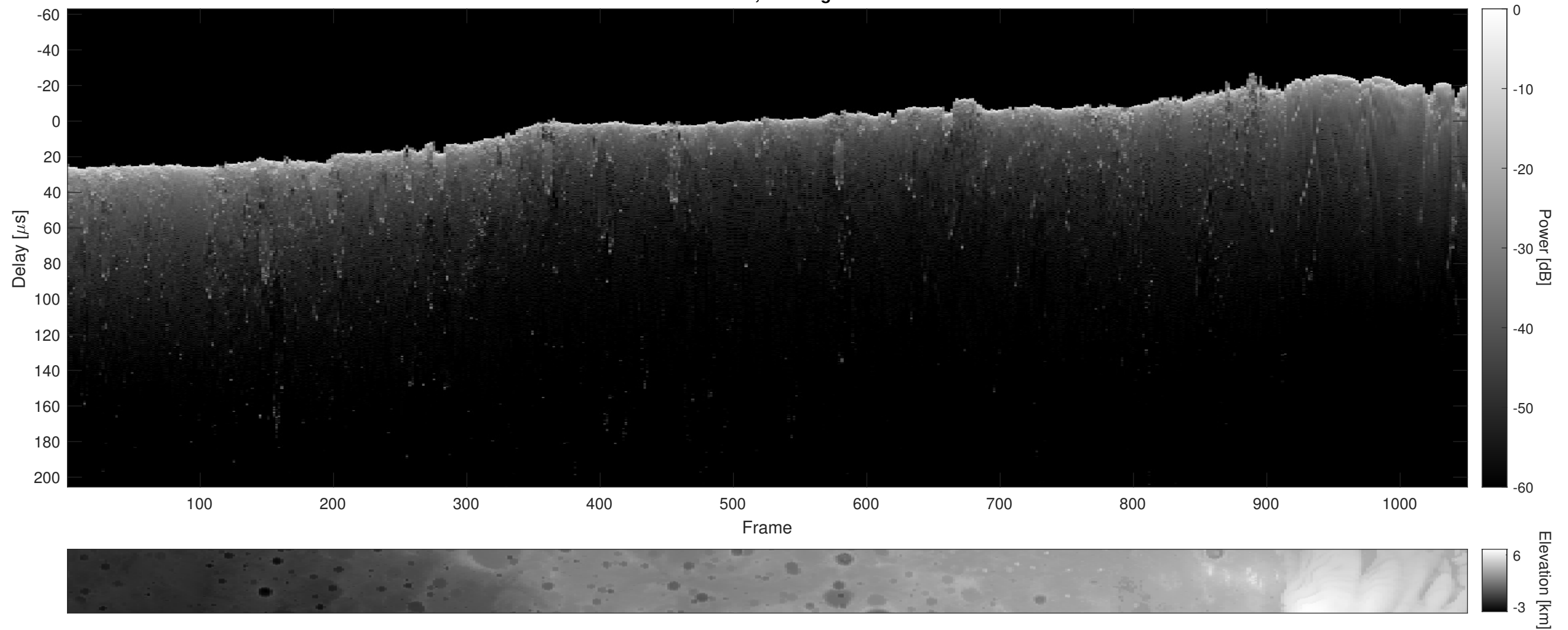
Orbit 2806, Cluttergram
