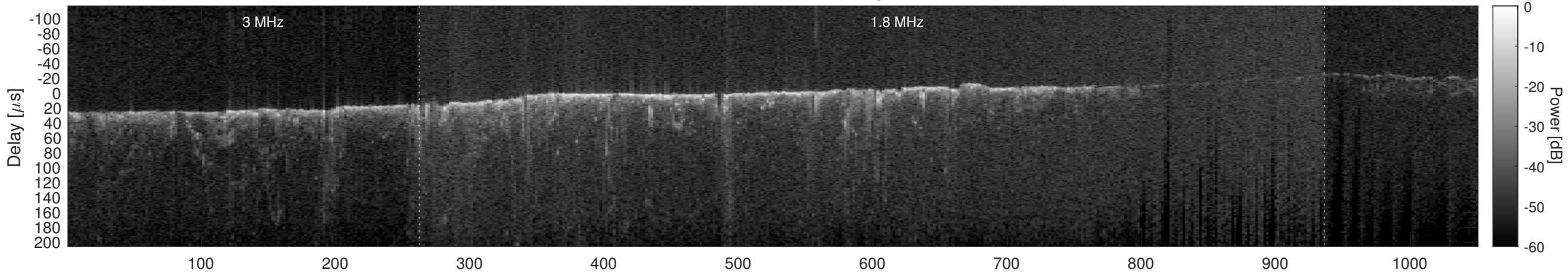
Orbit 2806, Cluttergram
