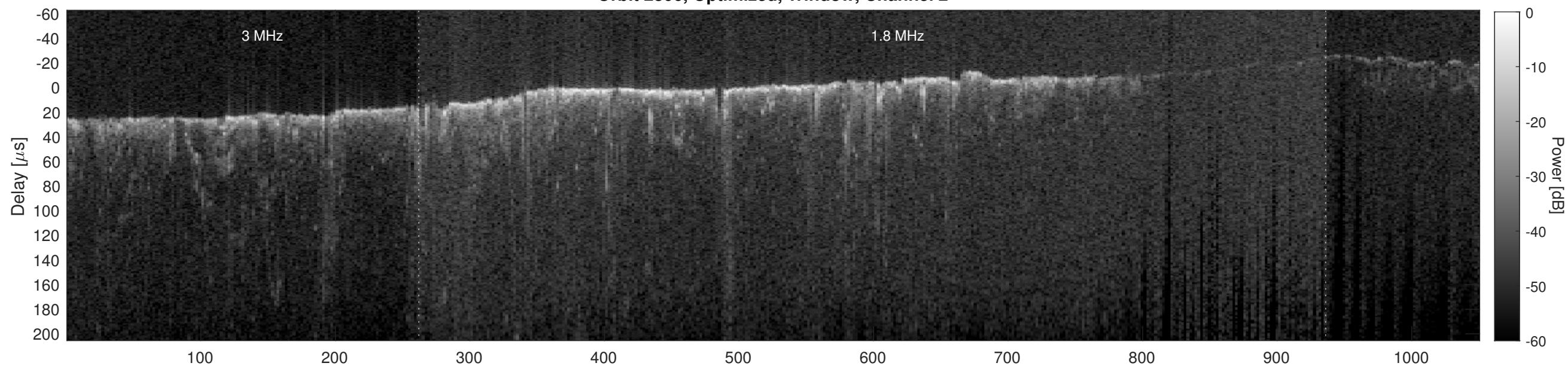
Orbit 2806, Cluttergram
