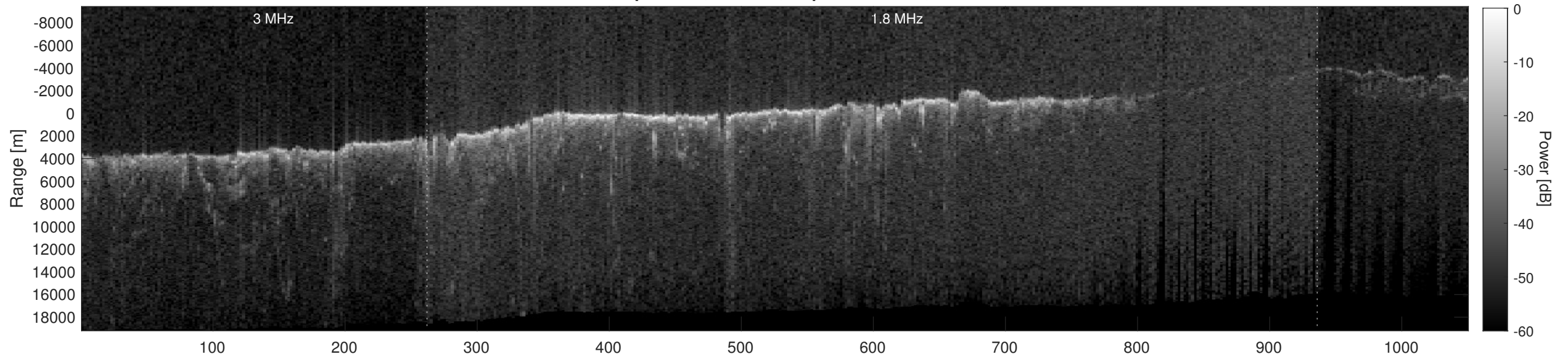
Orbit 2806, Depth-Corrected Cluttergram
