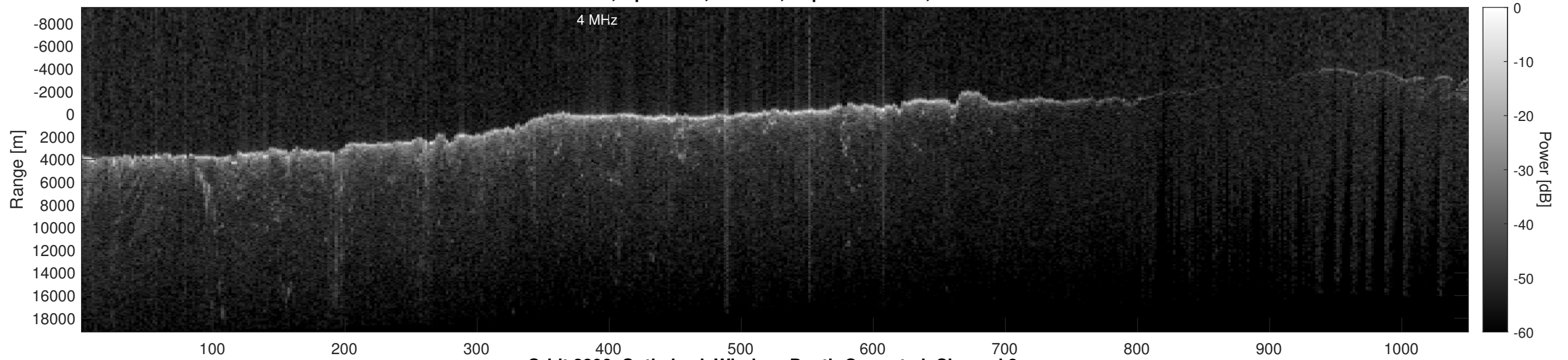
Orbit 2806, Optimized, Window, Depth-Corrected, Channel 2
