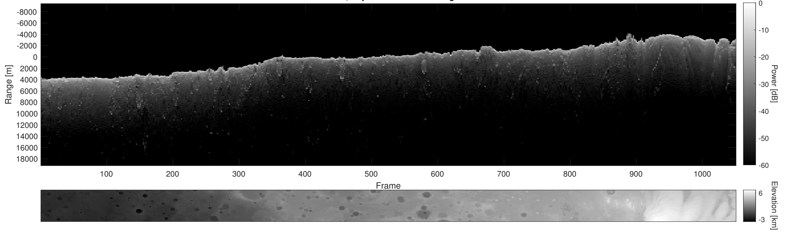
Orbit 2806, Depth-Corrected Cluttergram
