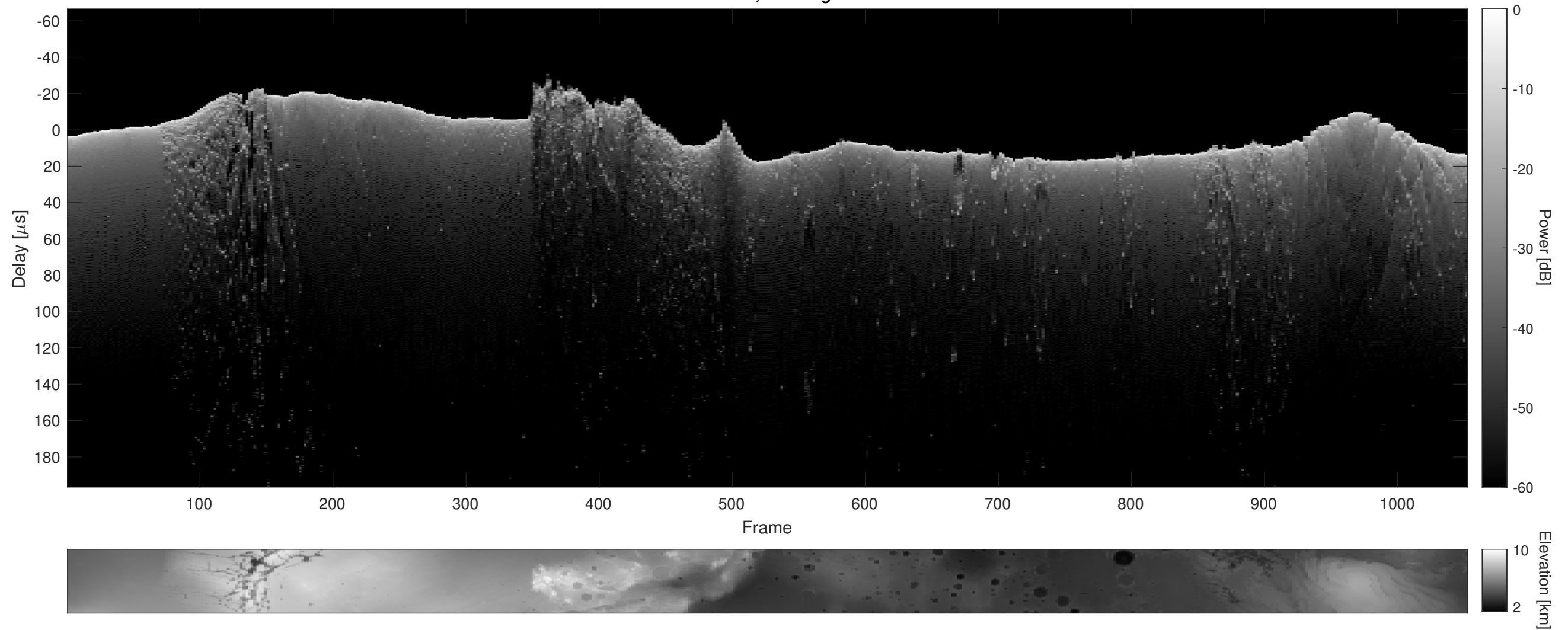
Orbit 2807, Cluttergram
