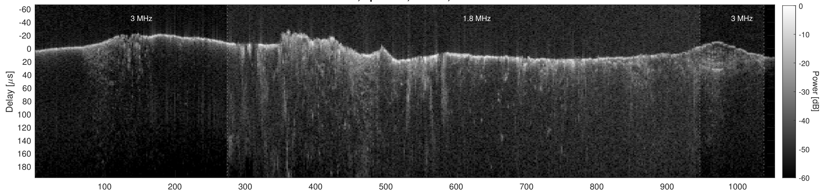
Orbit 2807, Cluttergram
