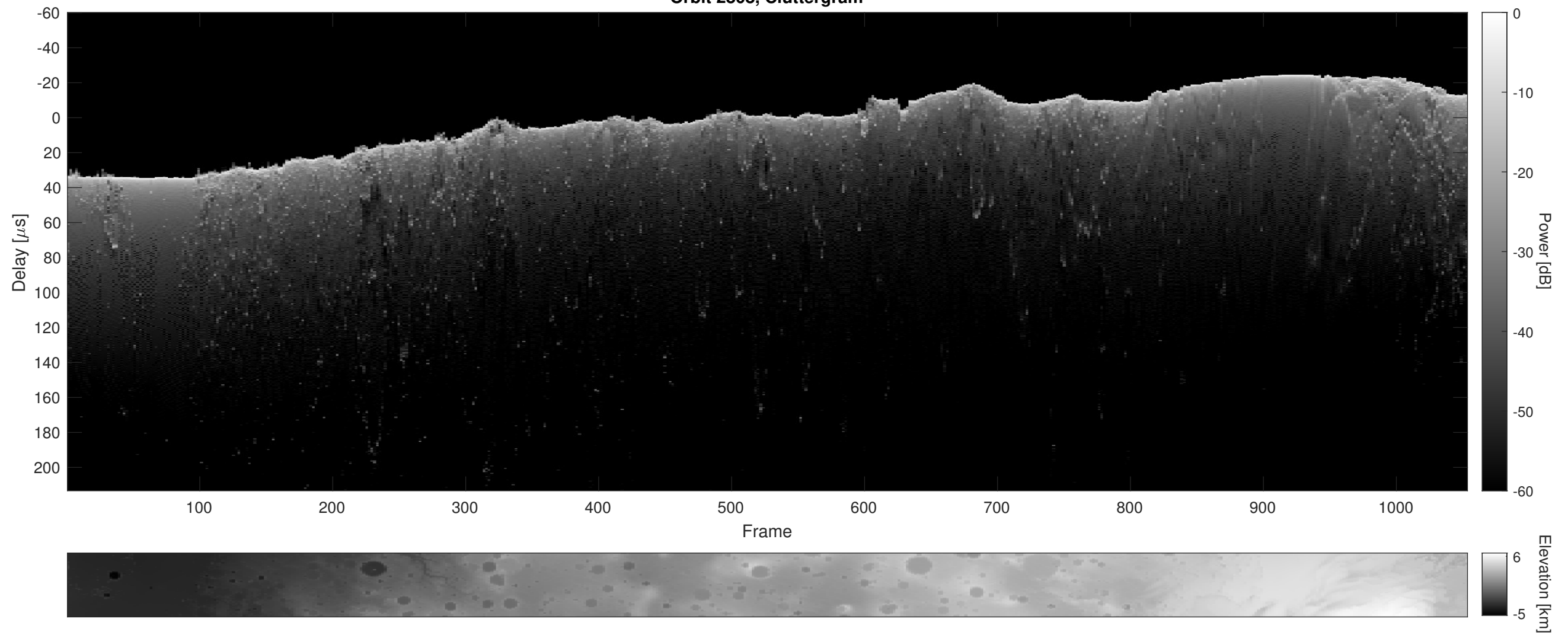
Orbit 2808, Cluttergram
