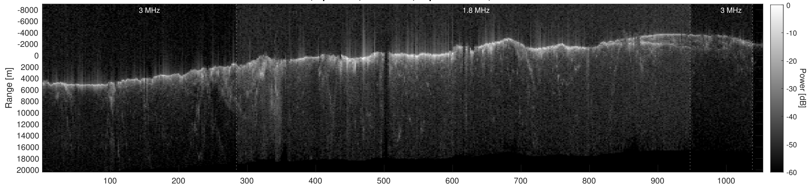
Orbit 2808, Depth-Corrected Cluttergram
