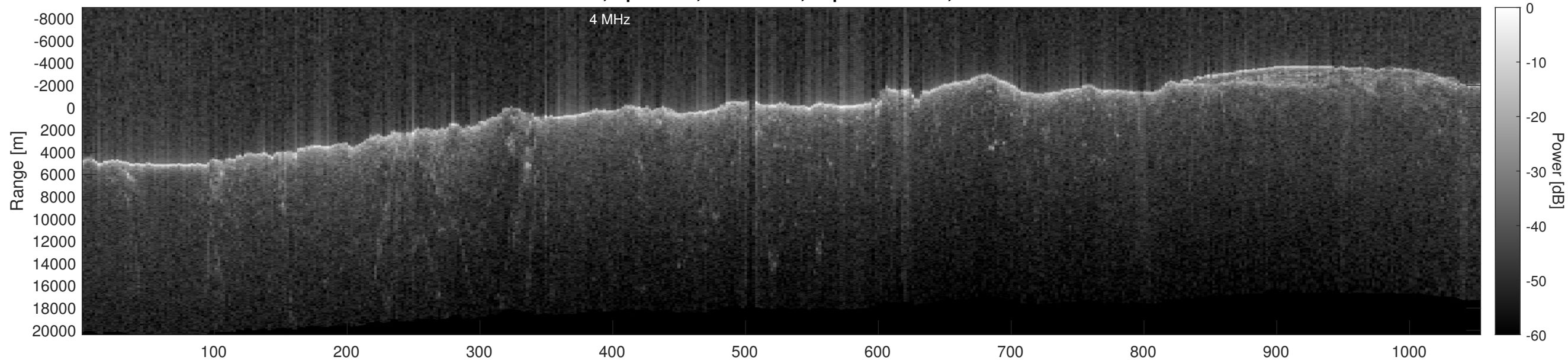
Orbit 2808, Optimized, No Window, Depth-Corrected, Channel 2
