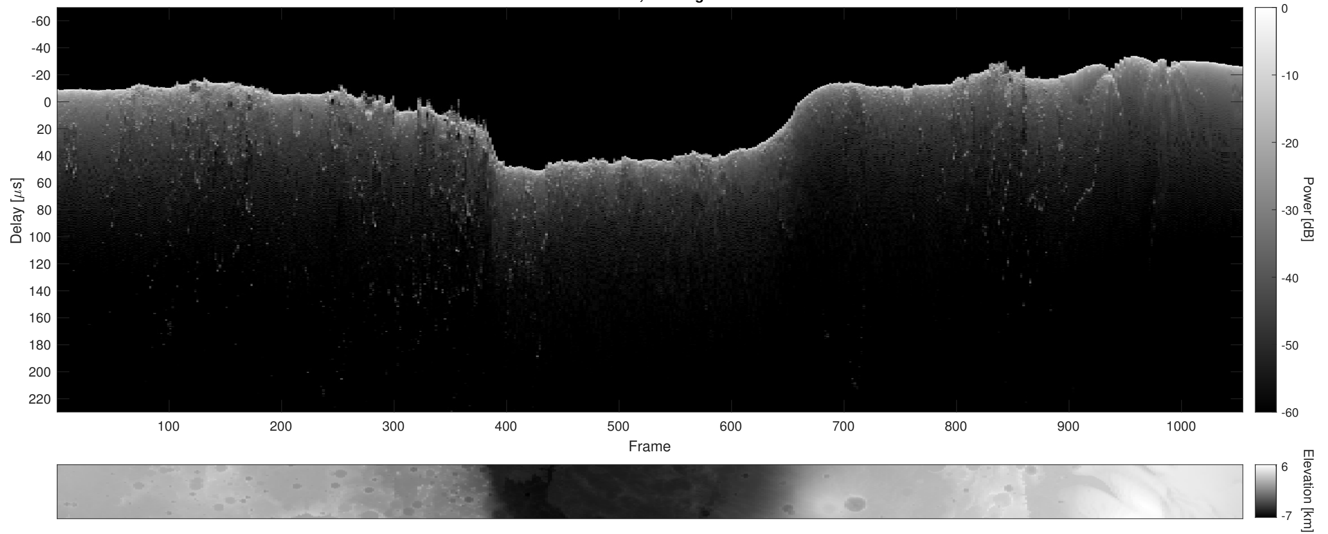
Orbit 2809, Cluttergram
