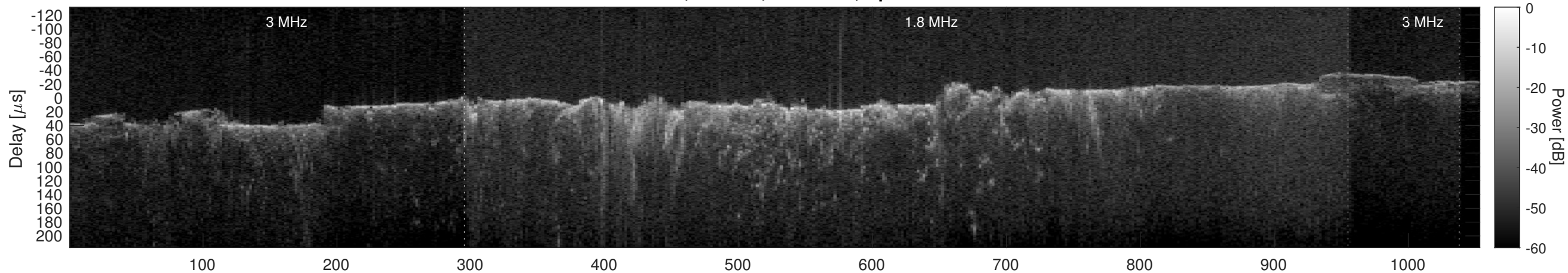
Orbit 2810, Cluttergram
