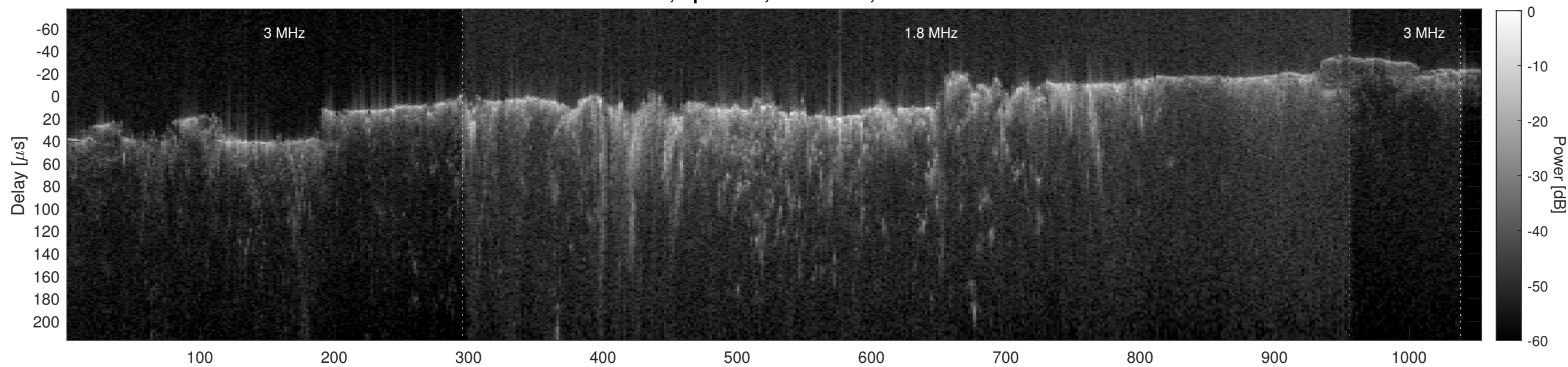
Orbit 2810, Cluttergram
