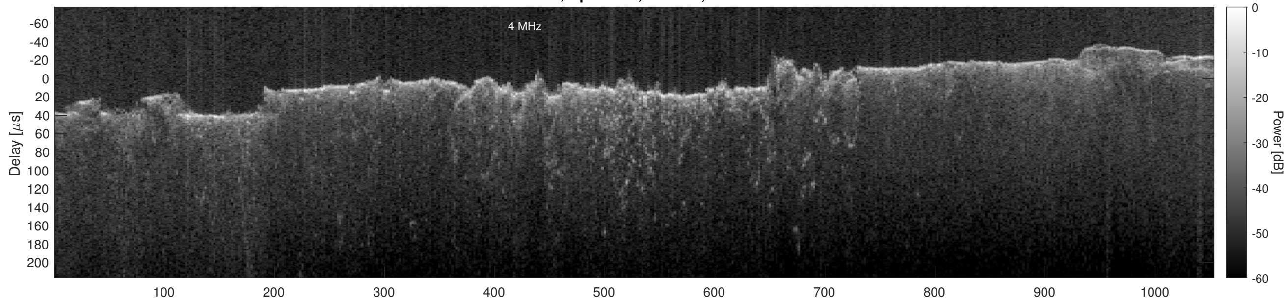
Orbit 2810, Optimized, Window, Channel 2
