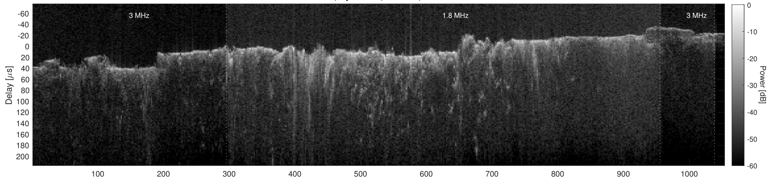
Orbit 2810, Cluttergram
