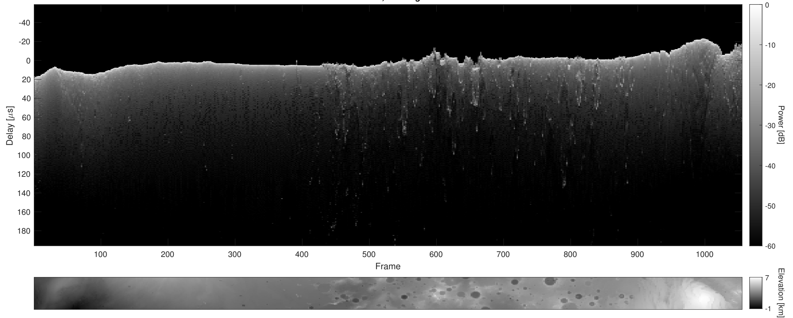
Orbit 2811, Cluttergram
