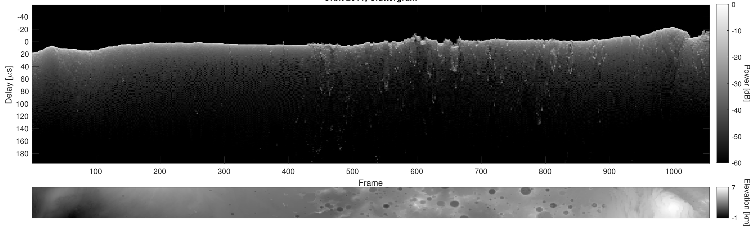
Orbit 2811, Cluttergram
