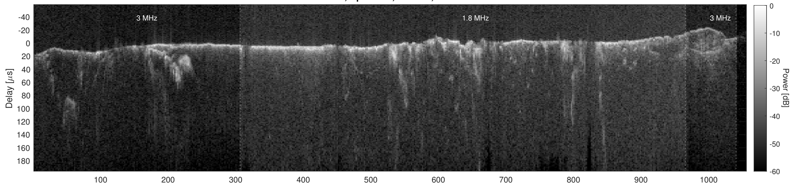
Orbit 2811, Cluttergram
