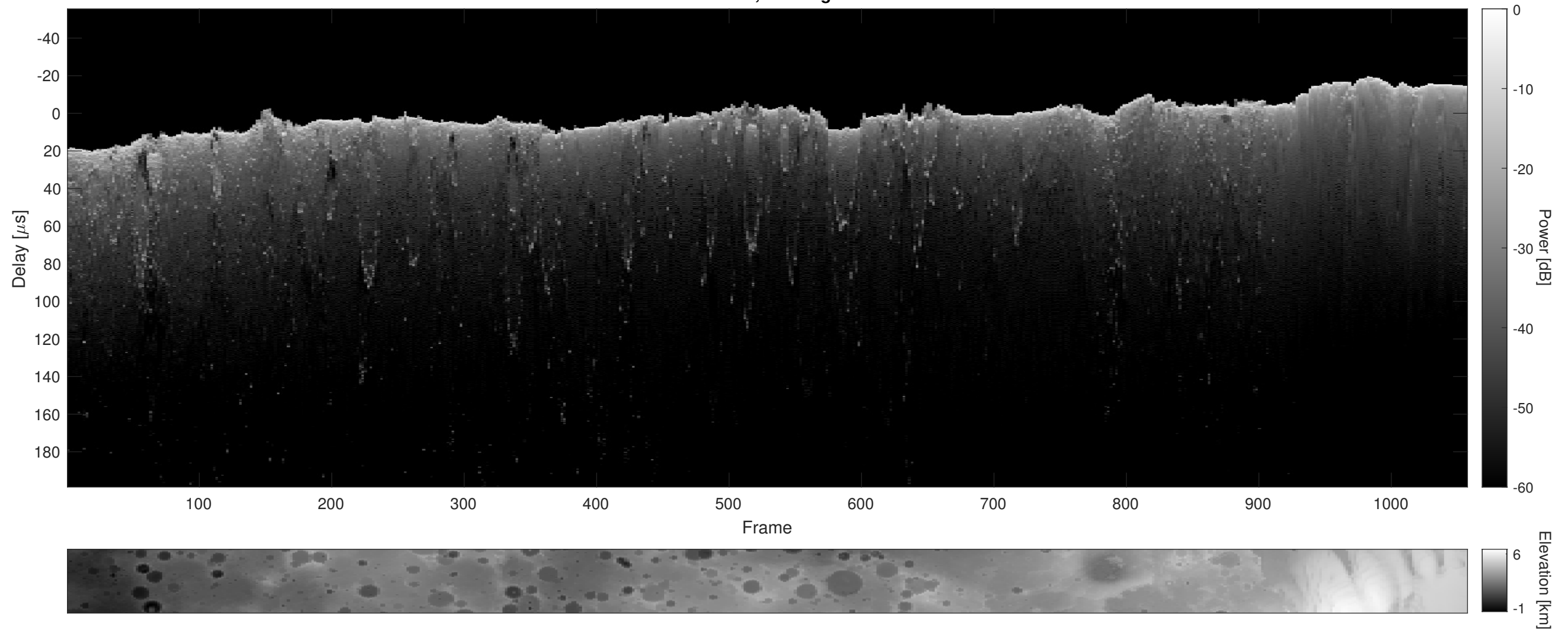
Orbit 2813, Cluttergram
