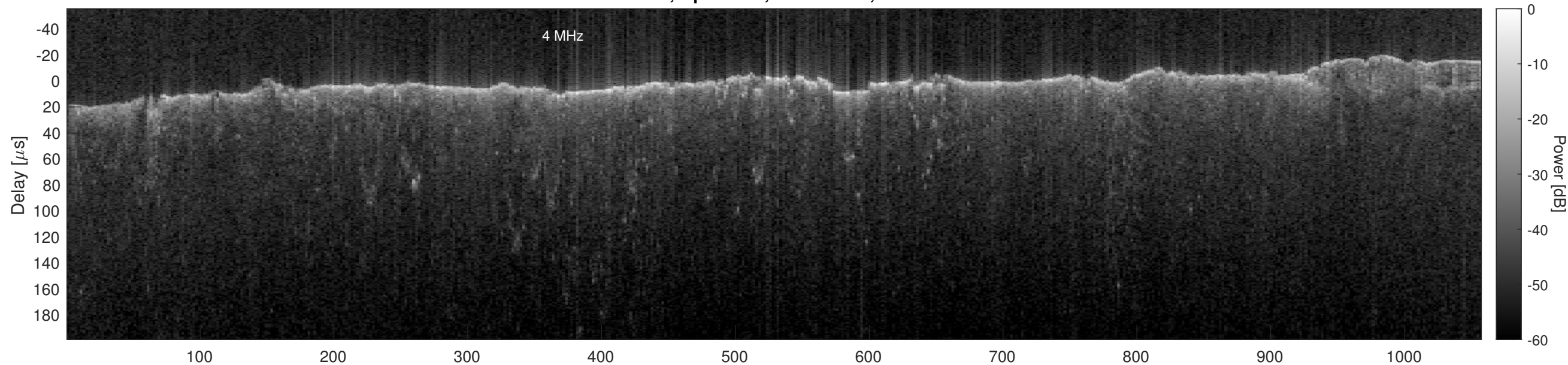
Orbit 2813, Optimized, No Window, Channel 2
