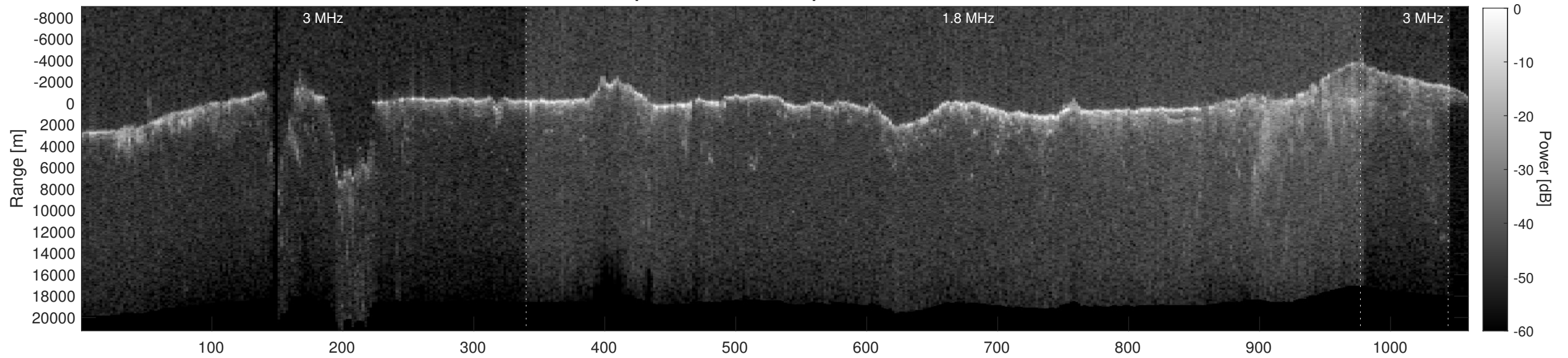
Orbit 2814, Depth-Corrected Cluttergram
