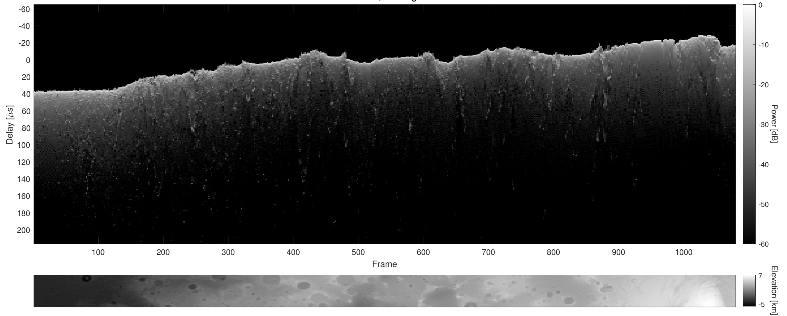
Orbit 2815, Cluttergram
