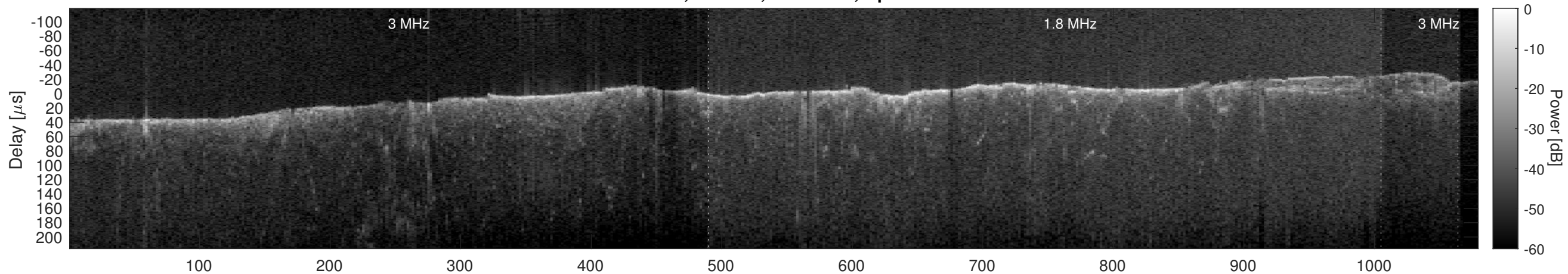
Orbit 2815, Cluttergram
