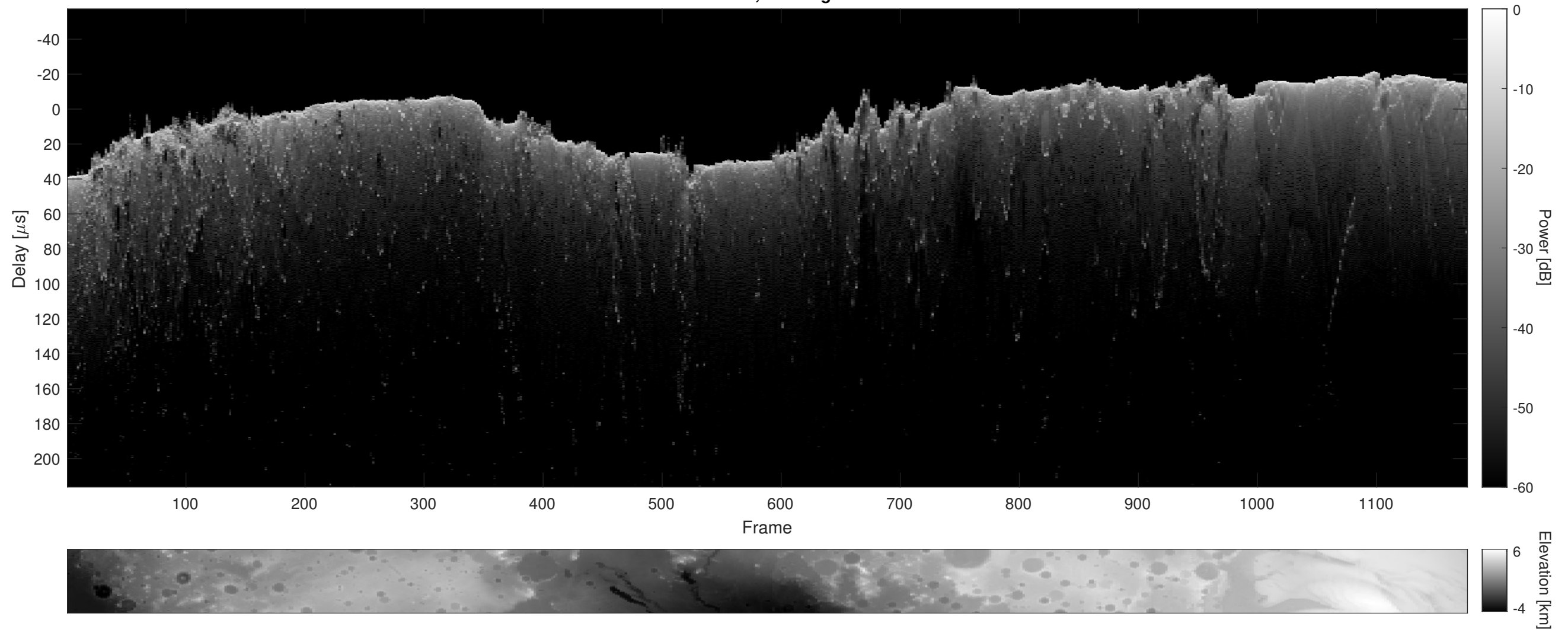
Orbit 2816, Cluttergram
