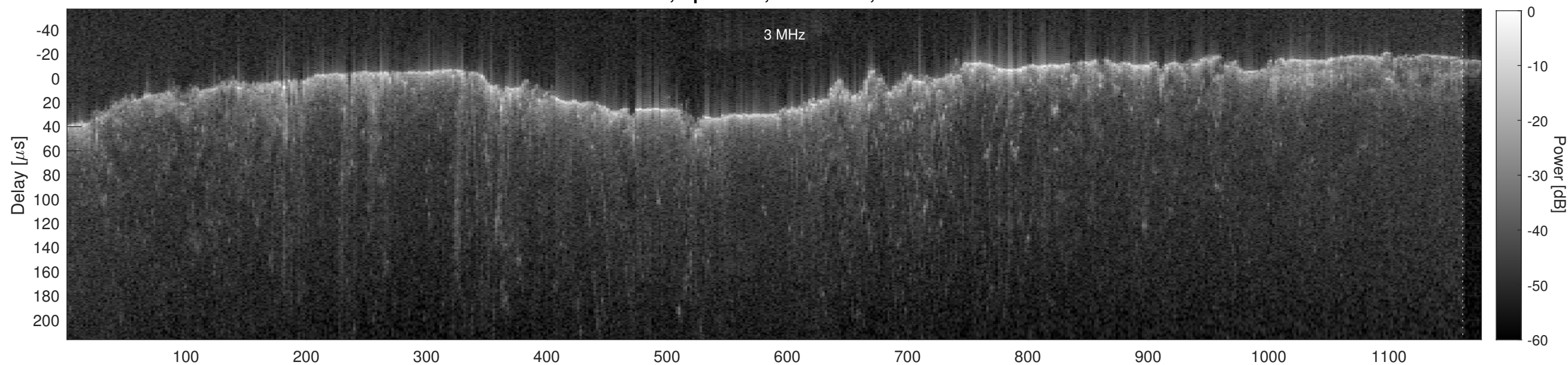
Orbit 2816, Cluttergram
