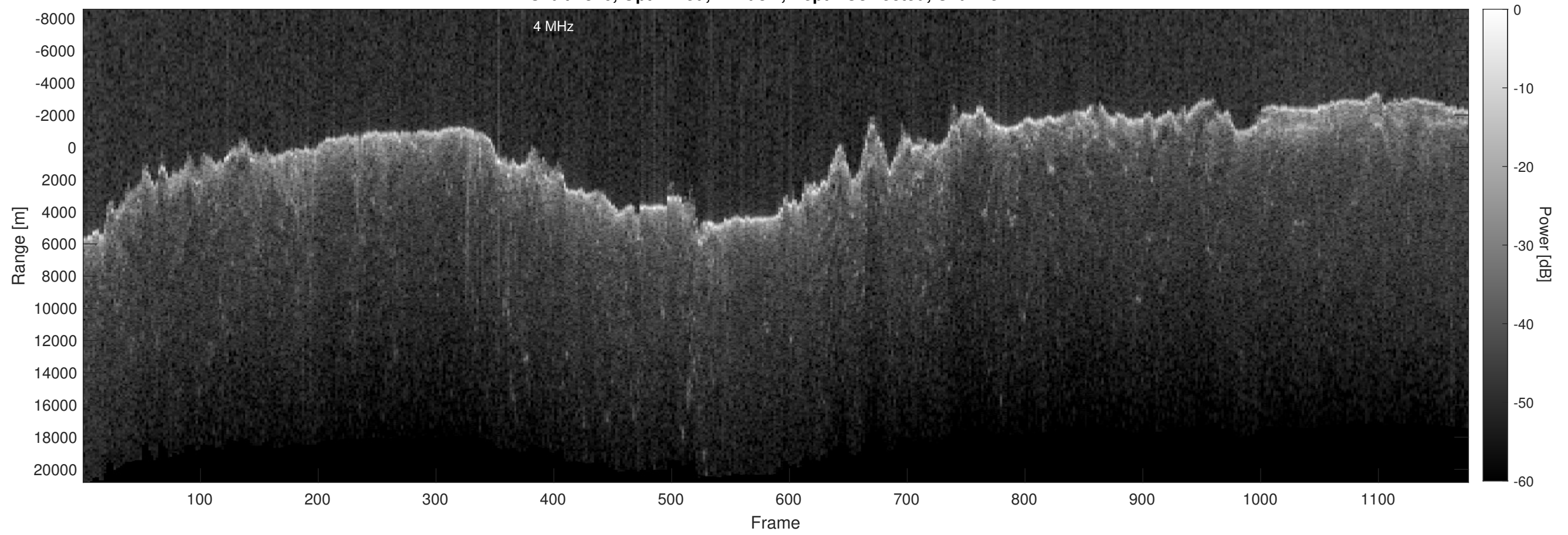
Orbit 2816, Optimized, Window, Depth-Corrected, Channel 2
