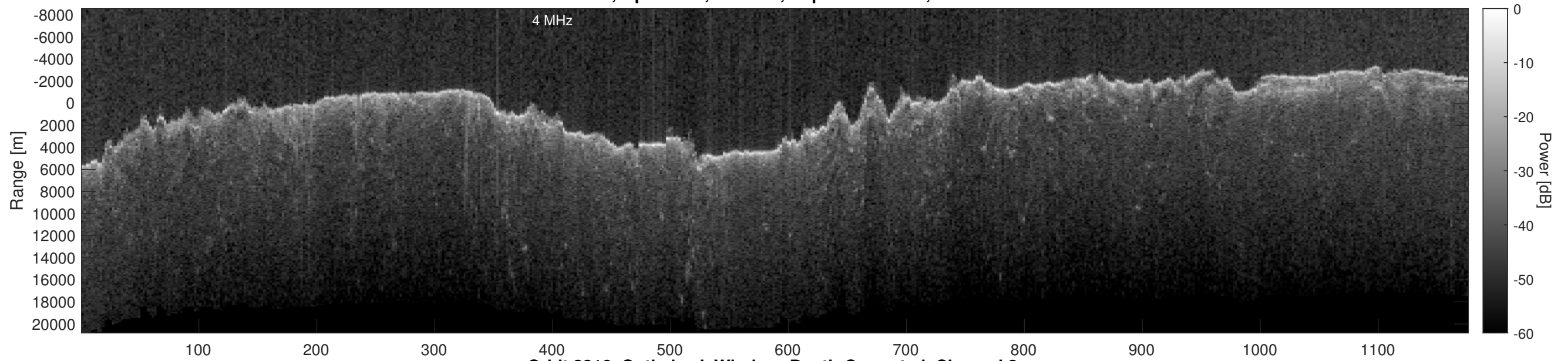
Orbit 2816, Optimized, Window, Depth-Corrected, Channel 2
