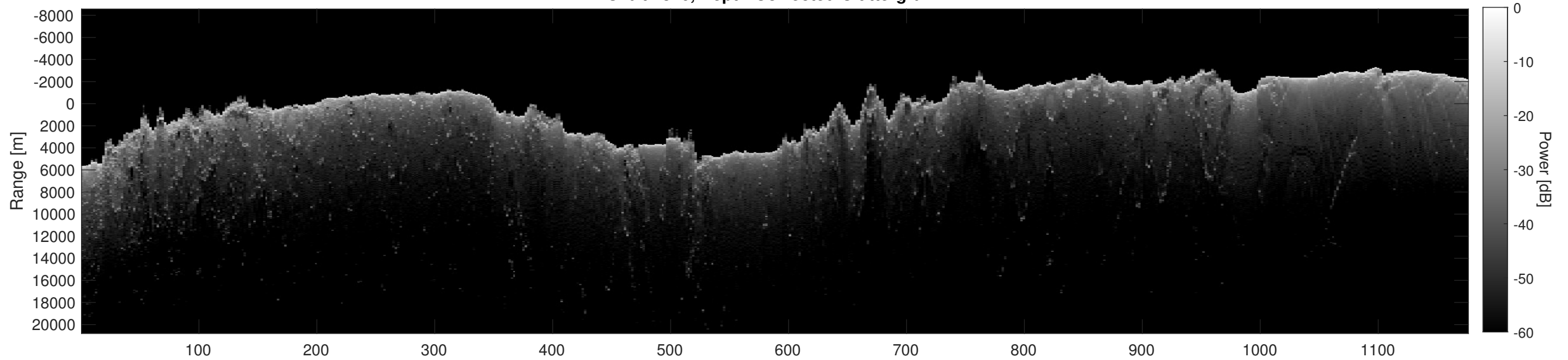
Orbit 2816, Depth-Corrected Cluttergram
