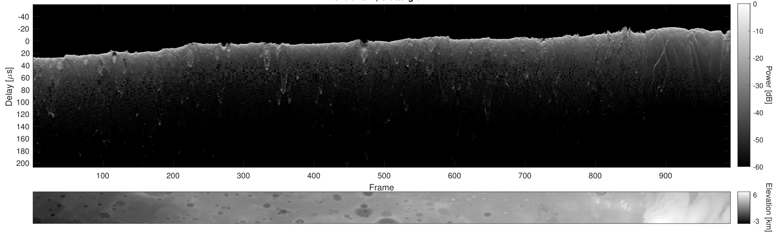
Orbit 2817, Cluttergram
