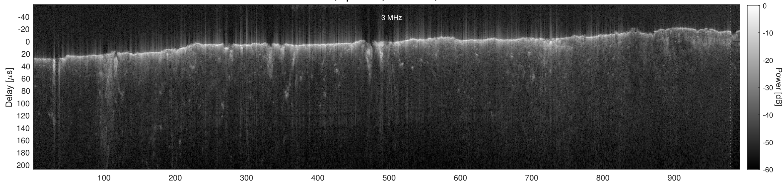
Orbit 2817, Cluttergram
