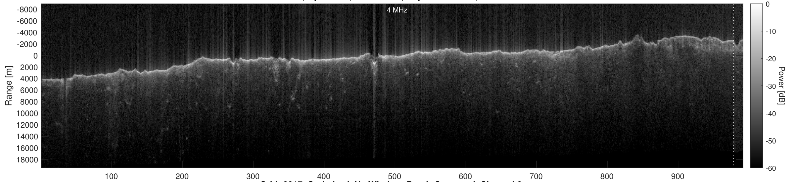
Orbit 2817, Optimized, No Window, Depth-Corrected, Channel 2
