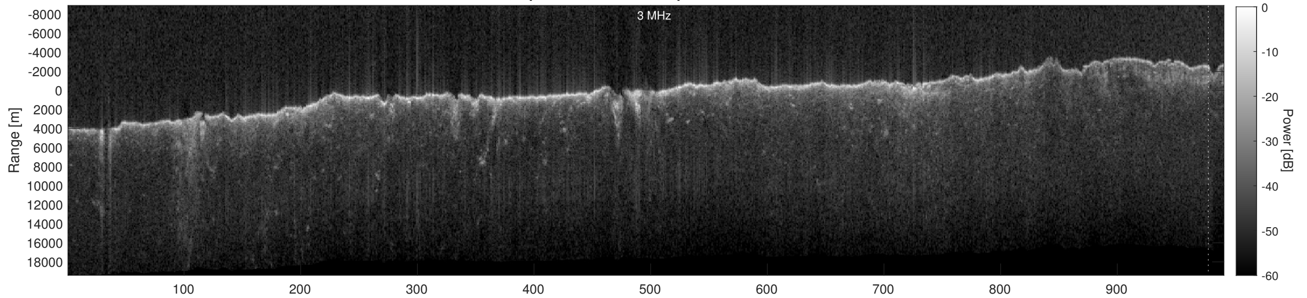
Orbit 2817, Depth-Corrected Cluttergram
