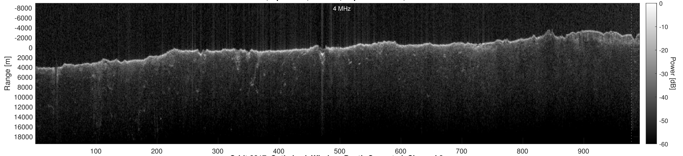
Orbit 2817, Optimized, Window, Depth-Corrected, Channel 2
