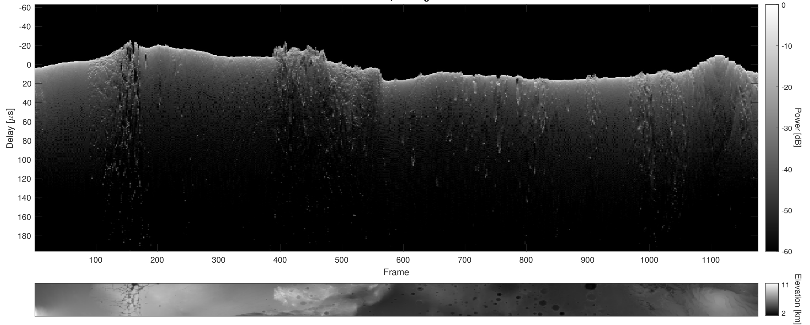
Orbit 2818, Cluttergram
