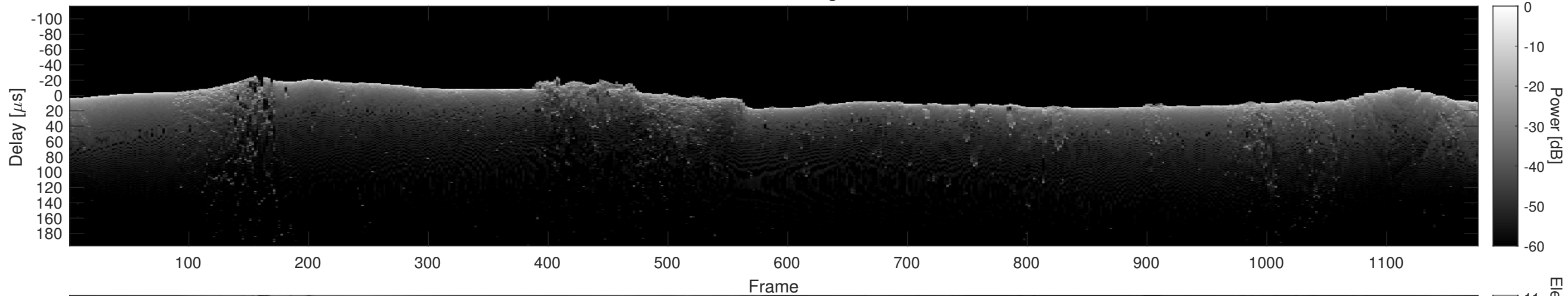
Orbit 2818, Cluttergram
