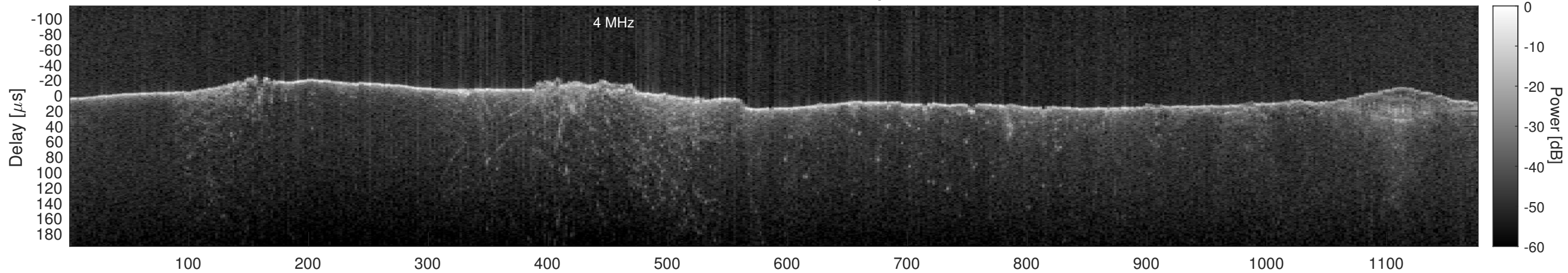
Orbit 2818, Cluttergram
