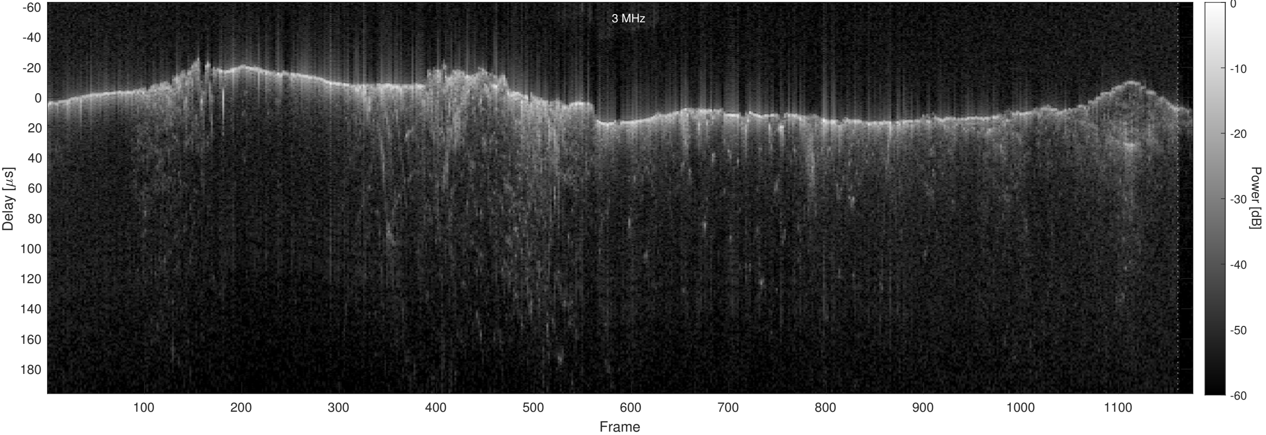
Orbit 2818, Optimized, No Window, Channel 2
