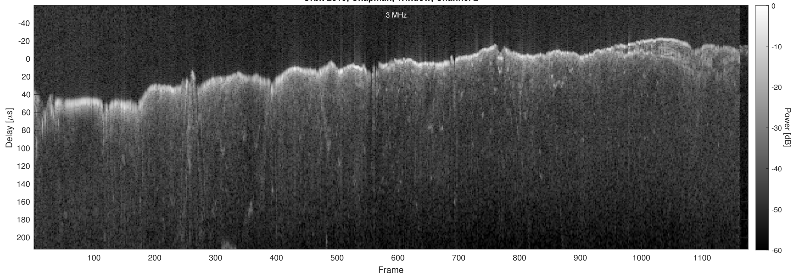
Orbit 2819, Chapman, Window, Channel 2
