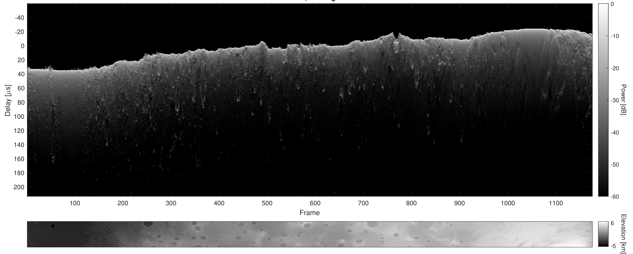
Orbit 2819, Cluttergram
