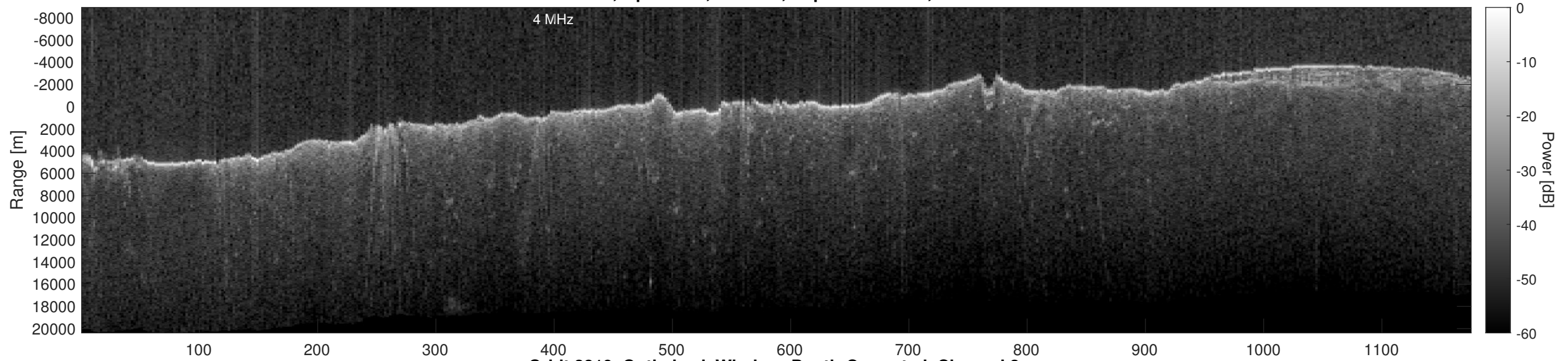
Orbit 2819, Optimized, Window, Depth-Corrected, Channel 2
