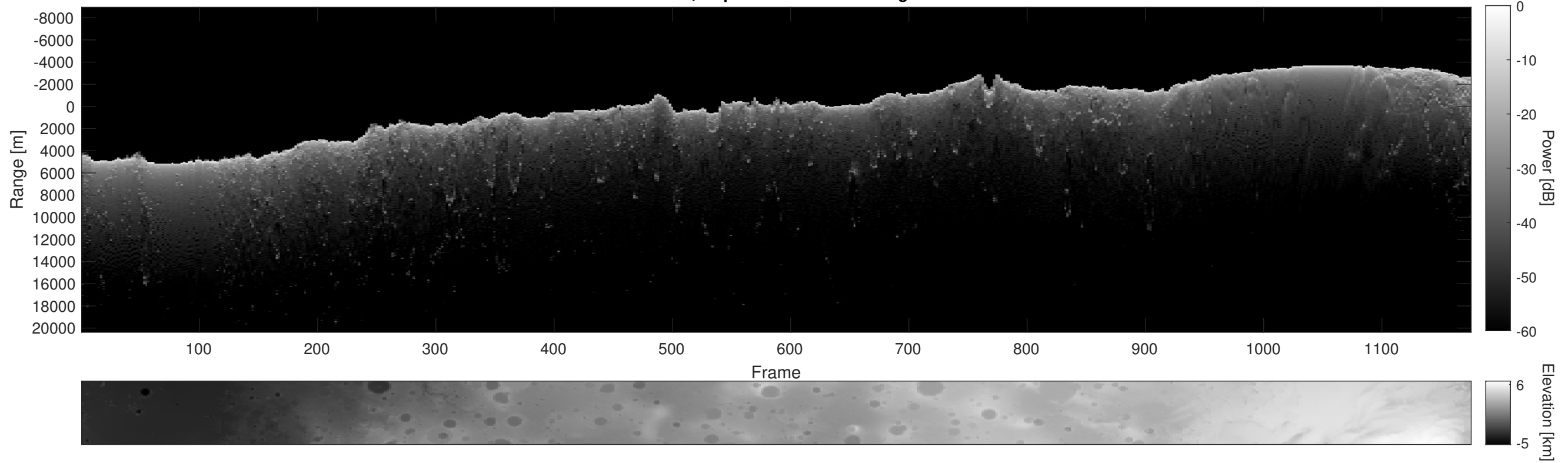
Orbit 2819, Depth-Corrected Cluttergram
