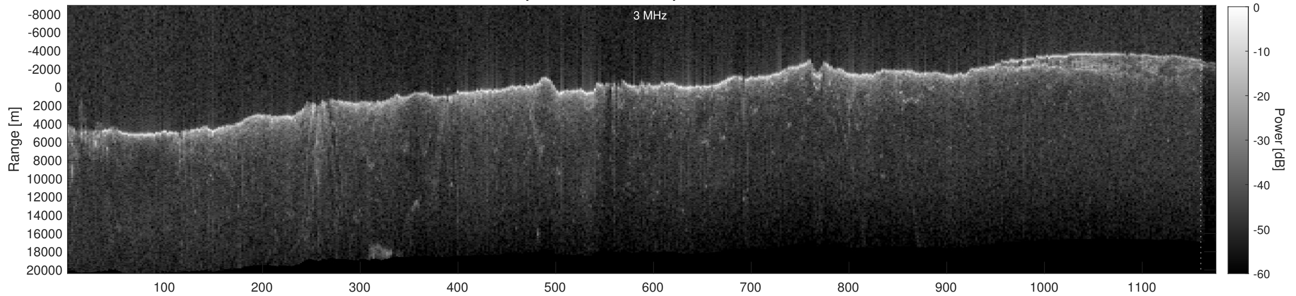
Orbit 2819, Depth-Corrected Cluttergram
