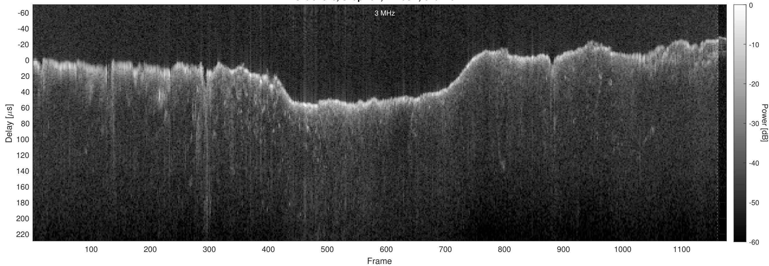
Orbit 2820, Chapman, Window, Channel 2
