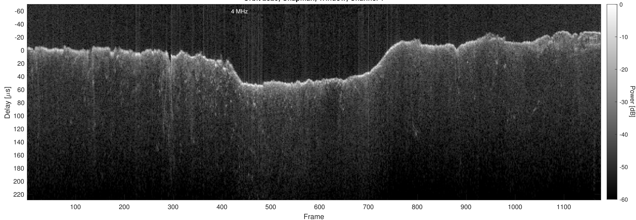
Orbit 2820, Chapman, Window, Channel 2
