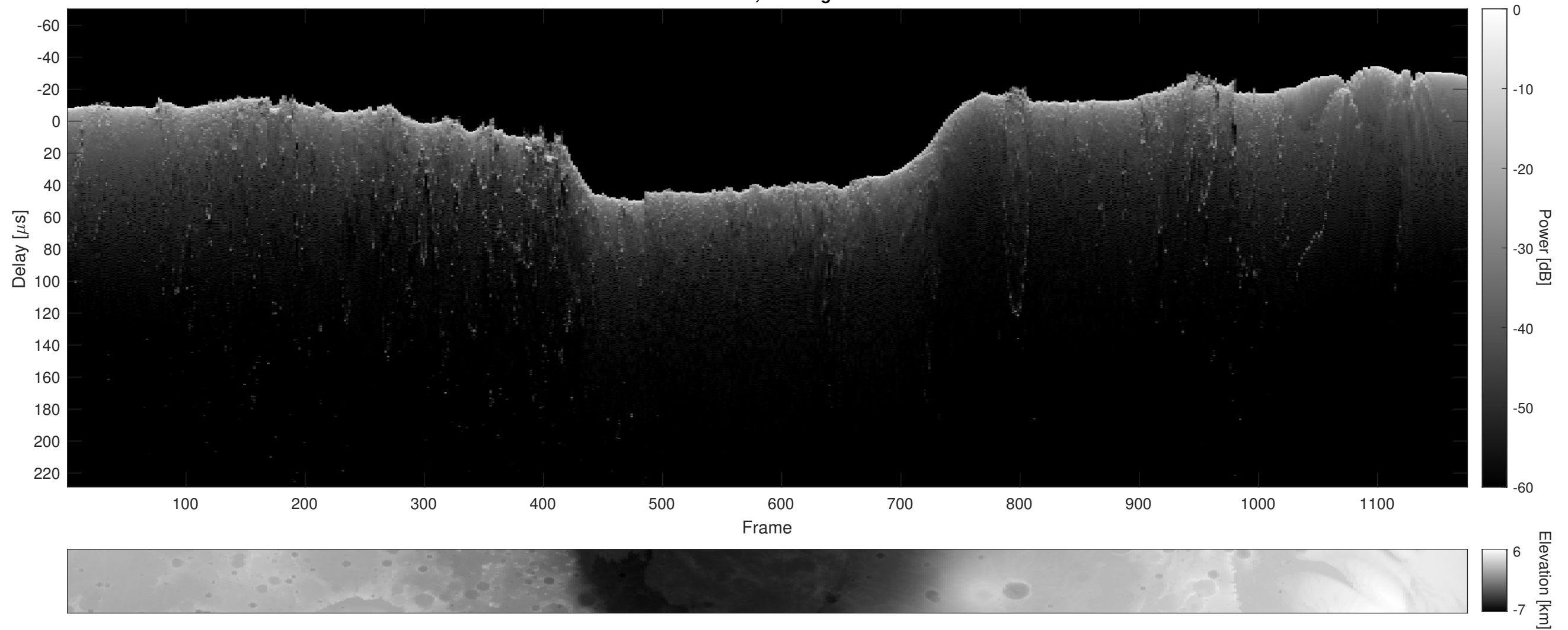
Orbit 2820, Cluttergram
