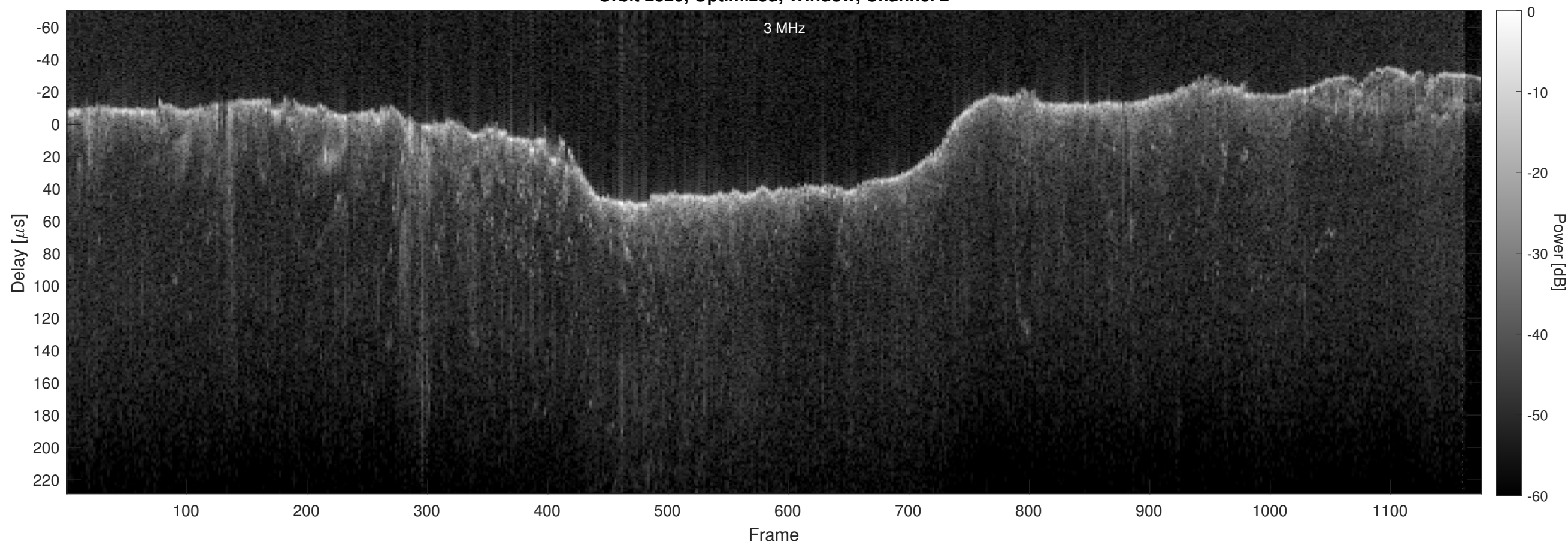
Orbit 2820, Optimized, Window, Channel 2
