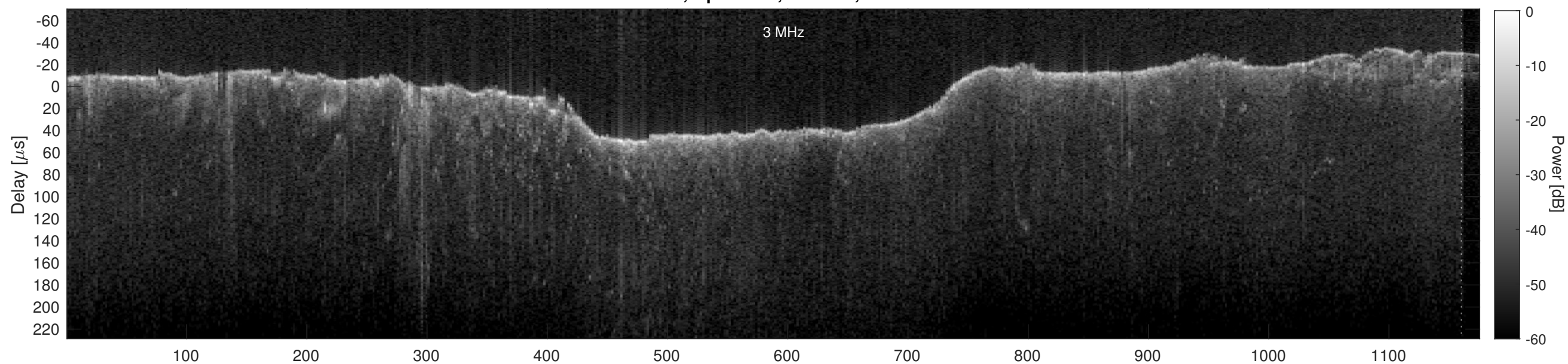
Orbit 2820, Cluttergram
