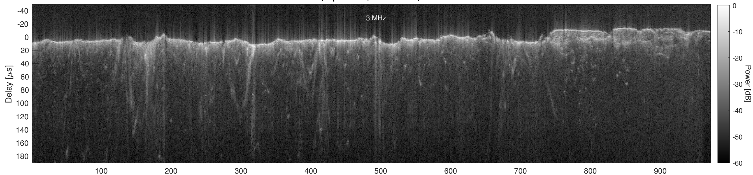
Orbit 2823, Cluttergram
