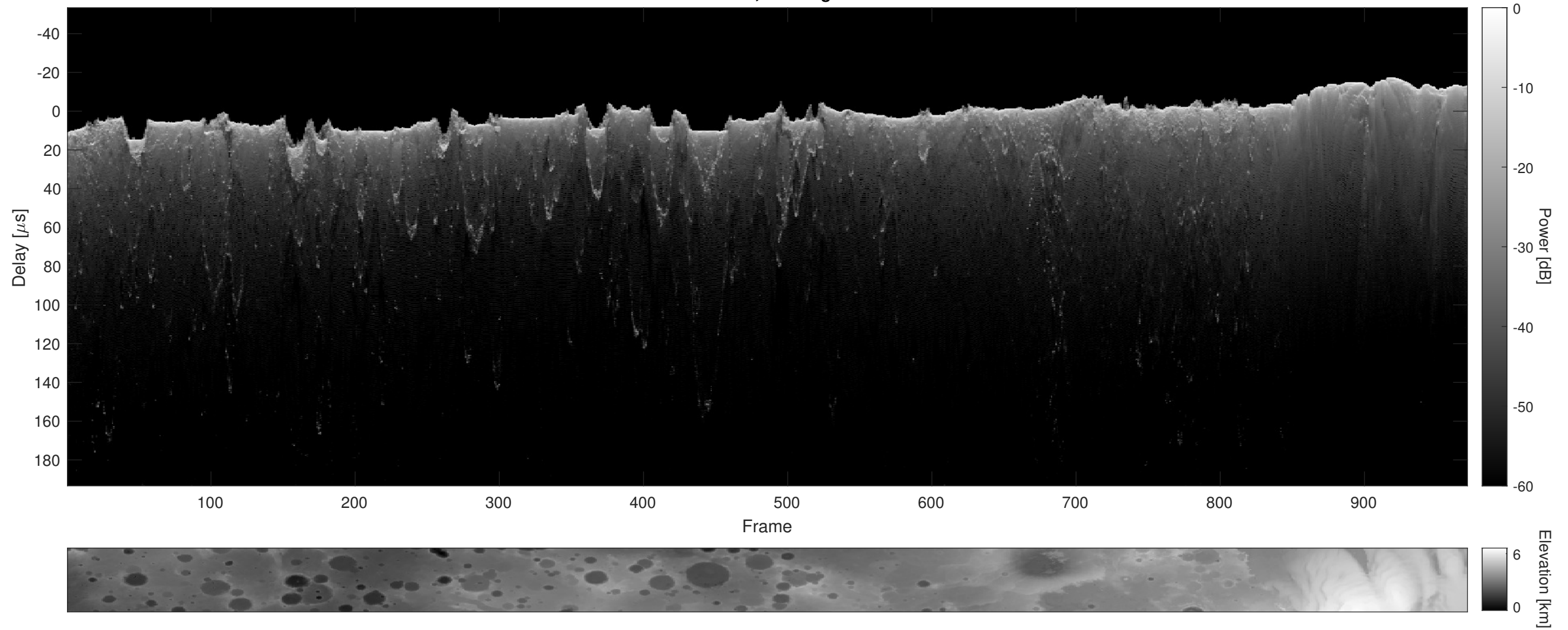
Orbit 2824, Cluttergram
