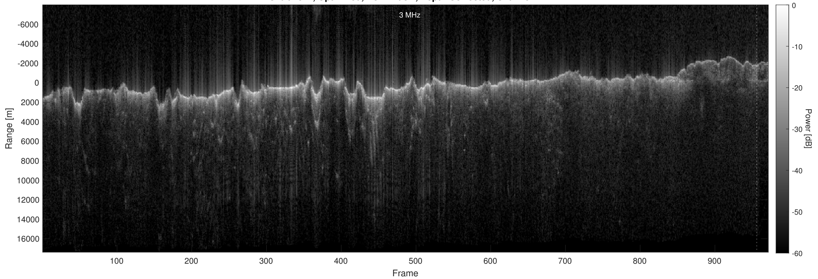
Orbit 2824, Optimized, No Window, Depth-Corrected, Channel 2
