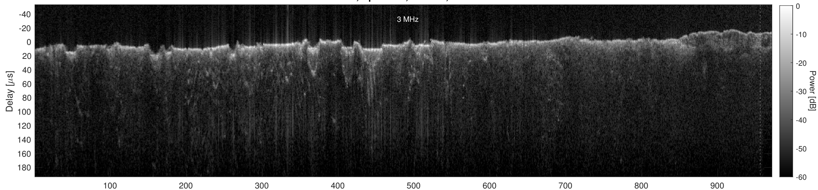
Orbit 2824, Cluttergram
