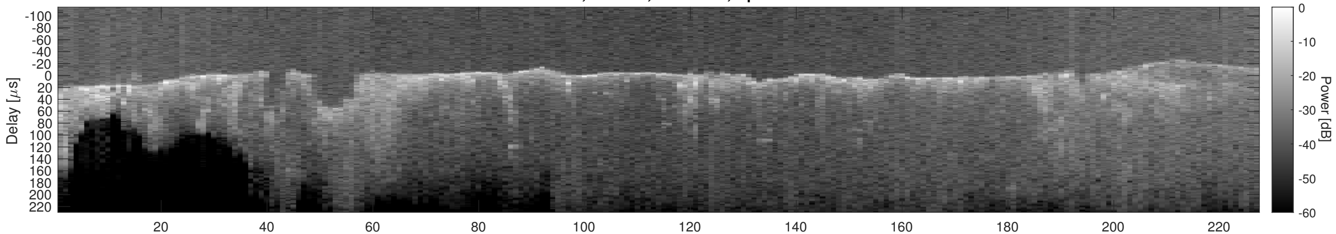
Orbit 2825, Cluttergram
