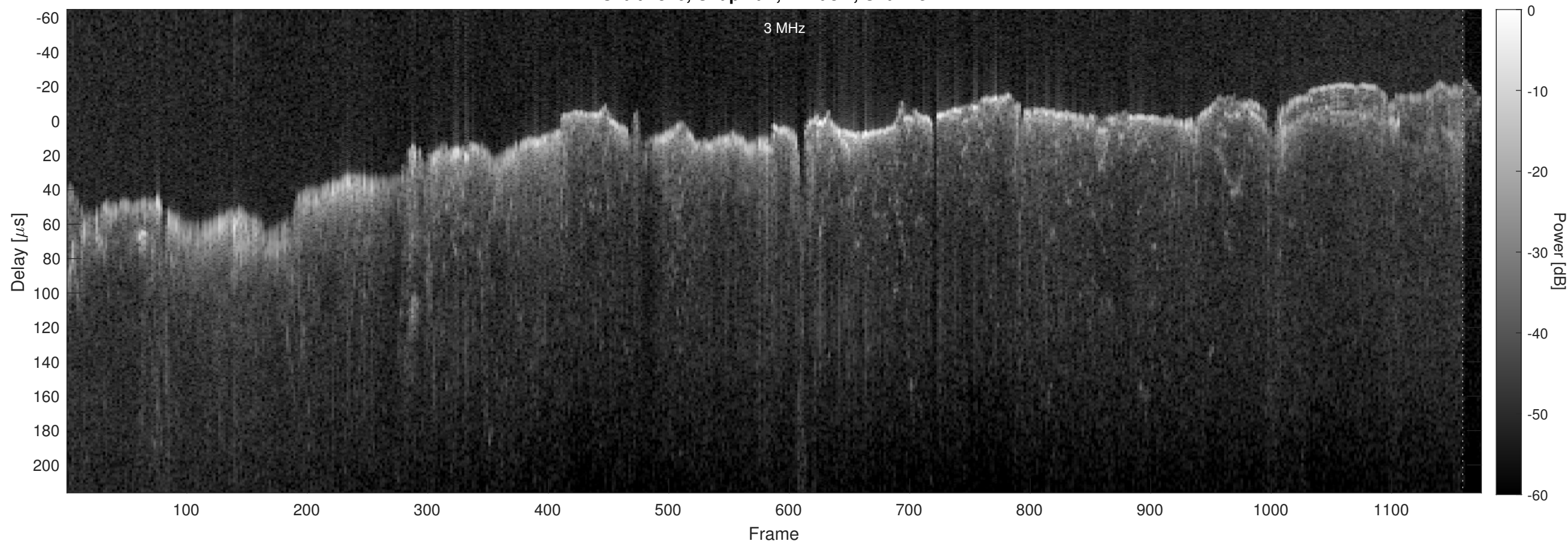
Orbit 2826, Chapman, Window, Channel 2
