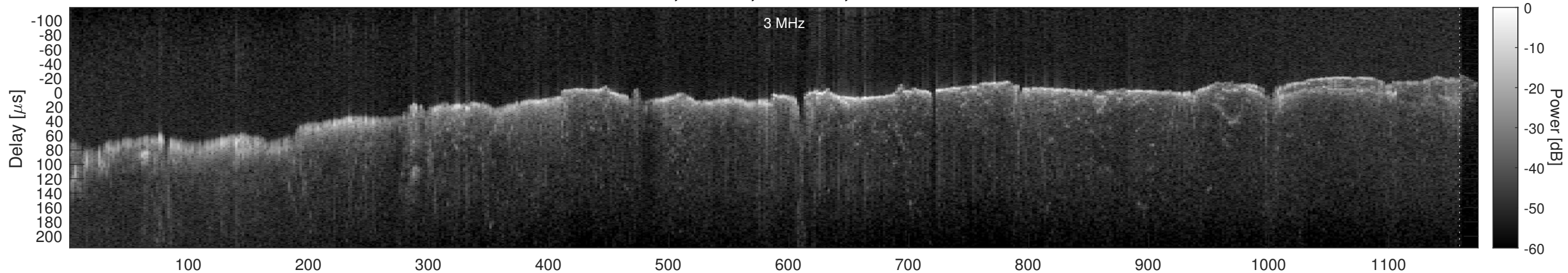
Orbit 2826, Window, Channel 2, Chapman
