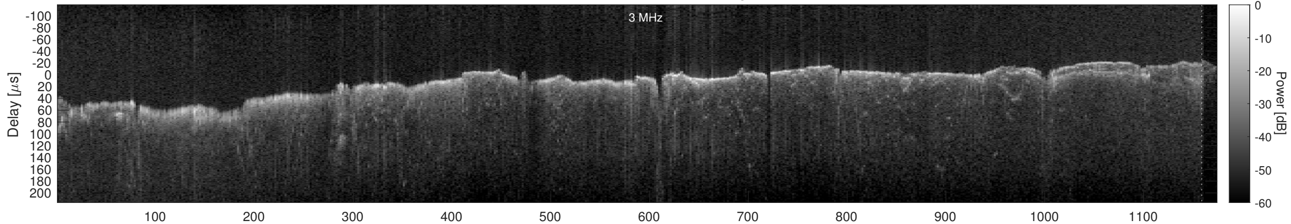
Orbit 2826, Window, Channel 2, Optimized
