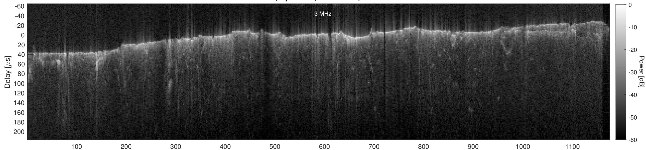
Orbit 2826, Cluttergram
